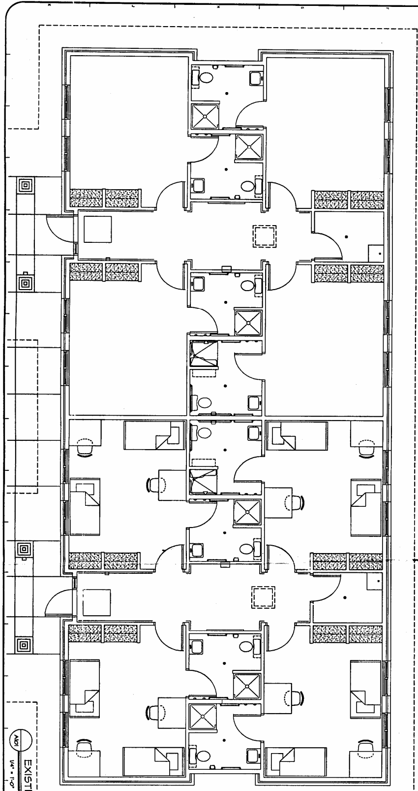
LINN STATE TECHNICAL COLLEGE HOUSING FLOOR PLAN
